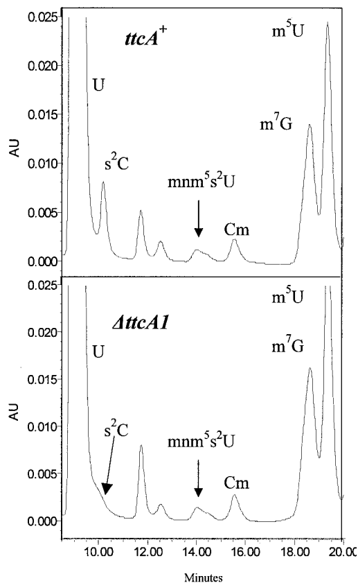
FIG. 1. HPLC chromatograms of tRNA hydrolysates from wild-type ttcA + (top) and the \Delta\text{ttcA1} mutant (bottom). The nucleosides were monitored at 254 nm. The positions of U, \text{s}^2\text{C} , \text{mnm}^5\text{s}^2\text{U} , Cm, \text{m}^7\text{G} , and \text{m}^5\text{U} are indicated. The arrow in the bottom panel denotes the position where \text{s}^2\text{C}32 should migrate if present. Only part of the chromatogram (5- to 25-min retention time) is shown.
