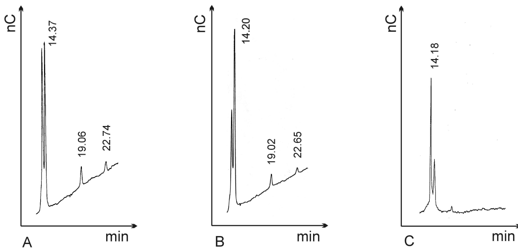
FIG. 3. Chromatographic separation of LMW succinoglycan. (A) Wild type; (B) tyrosine mutant RmΔPll15.pExoP-Y505S; (C) ATP-binding motif mutant RmΔPll15.pExoP-K589I. The monomer fraction eluted after 14 min, the dimer fraction eluted after 19 min, and the trimer fraction eluted after 22 min.
