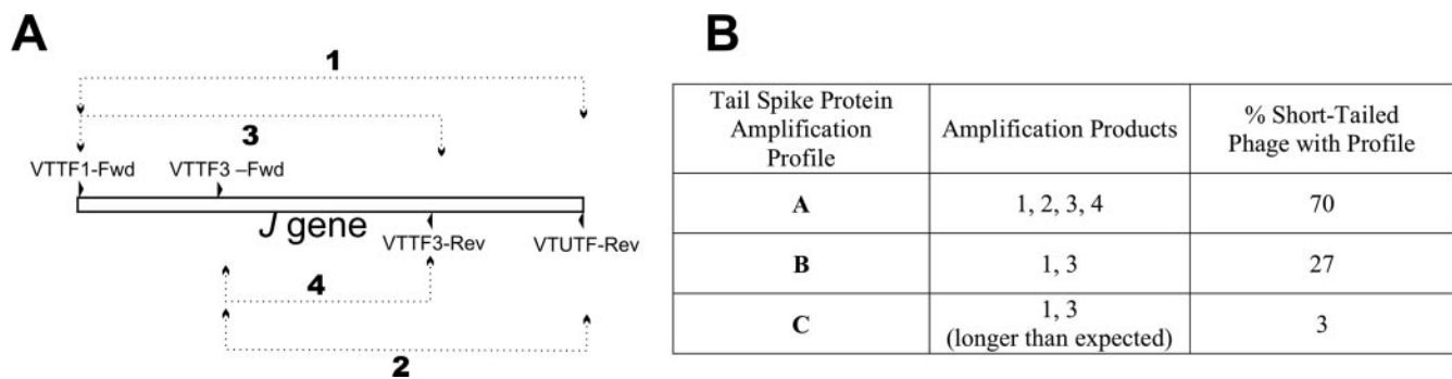
FIG. 8. Variations in tail spike proteins that recognize YaeT as an adsorption target. Amplification primers were designed against the gene sequence encoding the tail spike protein (the J gene orthologue) of \phi 24 B and 933W (VTTF1-Fwd, GTGTTGTTTCGGGGACG; VTUTF-Rev, TCATTCTCCTGTCTGCC; VTTF3-Fwd, TGCAGAGGAAAGCTCGAC; VTTF3-Rev, GCAGCCTCTTCTGCCTT). The primers were used in combinations of VTTF1-Fwd with VTUTF-Rev or VTTF3-Rev and of VTTF3-Fwd with VTUTF-Rev or VTTF3-Rev (combinations 1, 3, 2, and 4, respectively). All variations of tail spike proteins identified by this means were capable of adsorption to E. coli MC1061, and this adsorption could be blocked with the anti-YaeT sera. Three different amplification profiles were found for the short-tailed phages listed in the table in panel B. The majority (70%) of phages possessed amplification profile A, which results from the production of all four amplification products of the anticipated size. Profile C was found only rarely and is characterized by the failure of the VTUTF-Rev primer to produce any products in combination with either 5' primer, while the products of VTTF3-Rev were ~800 bp larger than expected.
