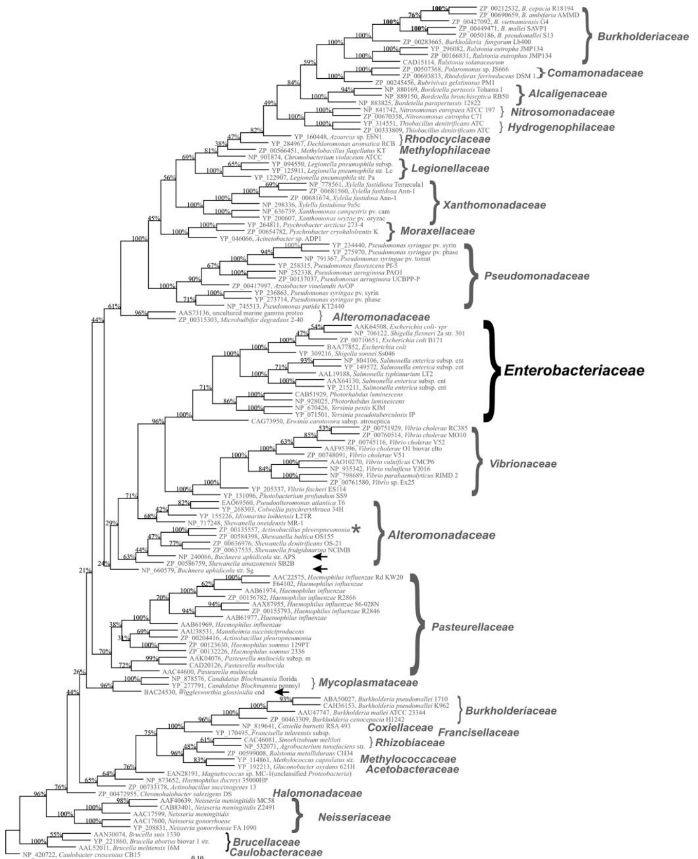
FIG. 2. Phylogenetic tree of YaeT orthologues for most of the gram-negative bacteria for which there are complete genome sequences. Homologues of YaeT were identified by BLASTP analyses and used to identify all homologues of YaeT possessing at least 30% amino acid identity. The sequences were aligned and then subjected to a maximum parsimony analysis using ARB (29). Branches were validated through 100 bootstrap analyses. Scale bar = 1% amino acid changes. The Enterobacteriaceae is indicated by larger type, and a few unusual members of this family are indicated by arrows. The asterisk indicates a bacterial species that clusters with an unrelated bacterial family.
