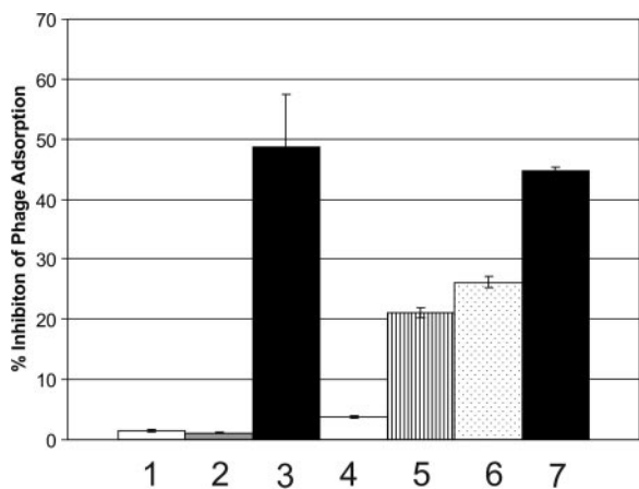
FIG. 5. Inhibition of \phi 24_B adsorption using rabbit anti-H-YaeT antiserum. A total of 5 \times 10^7 MC1061 cells were incubated with no serum (bar 1), rabbit preimmune serum (1:5 dilution) (bar 2), or rabbit anti-H-YaeT serum (1:5 dilution) (bar 3) prior to infection with \phi 24_B ( 5 \times 10^8 PFU). The error bars indicate the standard errors of the means ( n = 15 ). In a separate experiment, using the same numbers of cells and phage, various dilutions of the anti-H-YaeT serum were added to the cells prior to infection with \phi 24_B (bar 4, none; bar 5, 1:60 dilution; bar 6, 1:60 dilution; bar 7, 1:6 dilution) The error bars indicate the standard errors of the means ( n = 5 ).
