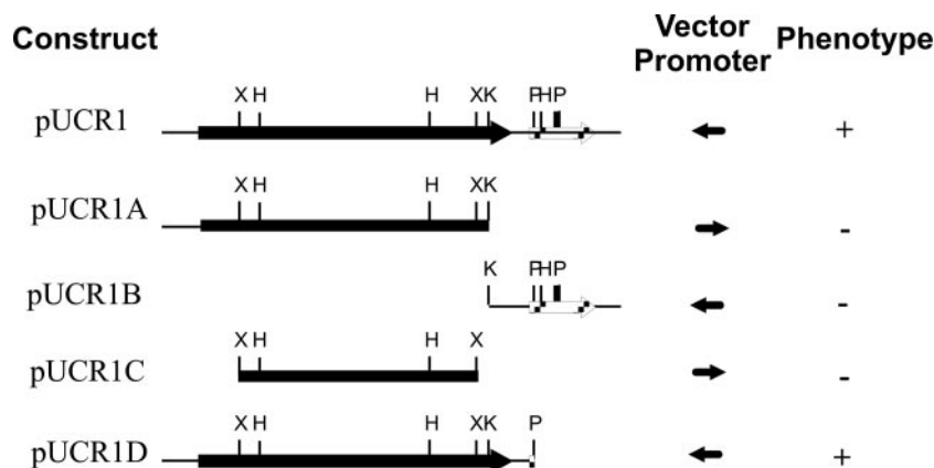
FIG. 1. Subcloning of the open reading frame associated with adsorption of \phi 24 B to MRL1. Construct pUCR1 was one of the four original clones that complemented the \phi 24 B phage adsorption defect. All four clones shared the two open reading frames present in pUCR1; the solid box represents yaeT , and the striped box represents skp . When fragments from pUCR1 were subcloned into pUC19 or pUC18 (indicated by the vector promoter direction: leftward, pUC19; rightward, pUC18), only the complete yaeT gene found in pUCR1 and pUCR1D complemented the MRL1 adsorption defect. Restriction sites are as follows: X, XhoI; H, HincII; K, KpnI; P, PstI.
