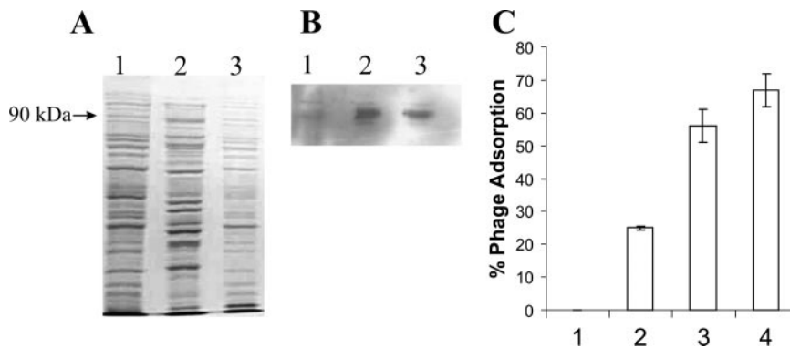
FIG. 6. Complementation of a natural yaeT mutant confers the ability to support \phi 24_B adsorption. (A) SDS-PAGE analysis of total cell protein from E. carotovora subsp. atroseptica (lane 2), E. coli strain MC1061 (lane 2), and E. carotovora subsp. atroseptica carrying the construct pKT230 yaeT (lane 3). The region corresponding to 90 kDa is indicated on the left. (B) Western blot analysis of total cell proteins from panel A. (C) Phage binding to YaeT on the surface of E. carotovora carrying pKT230 yaeT . Data were calculated for plasmid-free and pKT230-containing strains challenged with 3.4 \times 10^7 phage particles. The x axis indicates different total numbers of E. carotovora cells, as follows: bar 1, 1.5 \times 10^8 cells bearing pKT230; and bars 2, 3, and 4, 1.5 \times 10^8 , 3 \times 10^8 , and 5 \times 10^8 cells carrying pKT230 yaeT , respectively. The error bars indicate the standard errors of the means ( n = 5 ).
