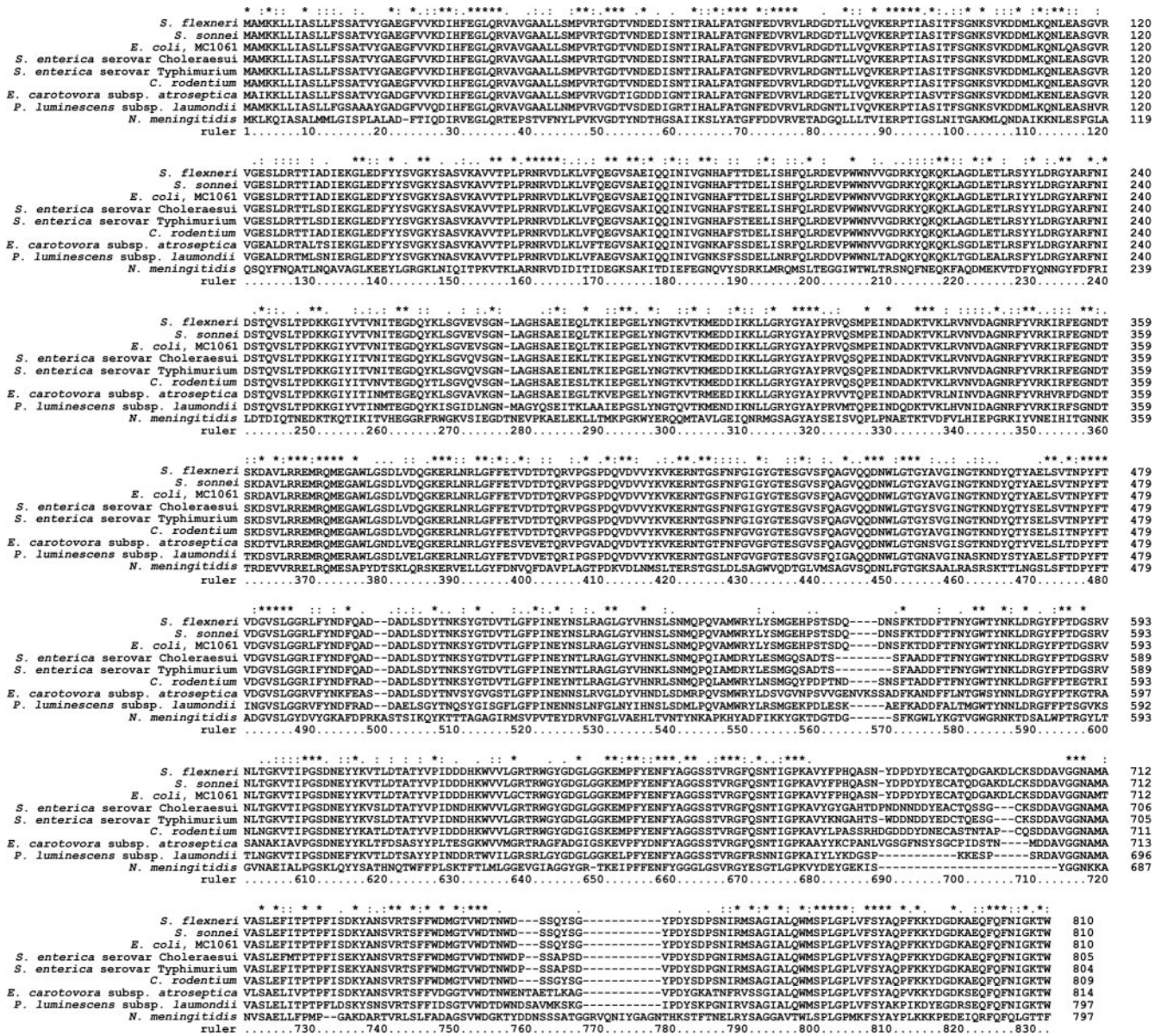
FIG. 3. Multiple alignment of YaeT from members of the Enterobacteriaceae . Clustal X (46) was used to align YaeT sequences from eight members of the Enterobacteriaceae against the orthologue from Neisseria meningitidis , for which a structure has been proposed (51). The alignments were used to identify regions possessing the greatest similarities and disparities; the latter are mostly associated with the carboxyl terminus and correspond to predicted extracellular loops. The conservation of residues is indicated above the alignments as follows: asterisk, complete identity; colon, conservation of a strong group (46); period, conservation of a weak group (46).
