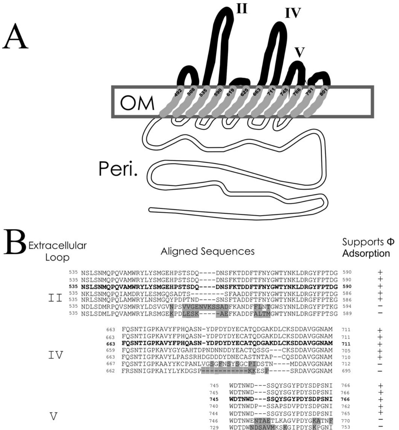
FIG. 7. Relationship between \phi 24 B phage adsorption and yaeT sequence variation with the predicted protein conformation in Enterobacteriaceae strains. (A) Proposed configuration of YaeT in the E. coli LPS membrane. The black loops are the predicted extracellular loops; the gray segments are predicted outer membrane (OM)-spanning regions; and the open segments are predicted periplasmic (Peri.) regions of YaeT. The extracellular loops are numbered from the amino terminus. (B) Identification of amino acid substitutions that correlate with the loss of Stx phage adsorption ability. The highlighted sequences are the changes predicted to be responsible for the loss of the ability to support phage adsorption. The sequences are sequences of, from top to bottom, S. flexneri , S. sonnei , E. coli strain MC1061, S. enterica serovar Choleraesuis strain SC-B67, C. rodentium strain ICC168, E. carotovora subsp. atroseptica strain SCR11043, and P. luminescens subsp. laumondii strain TTO1.
