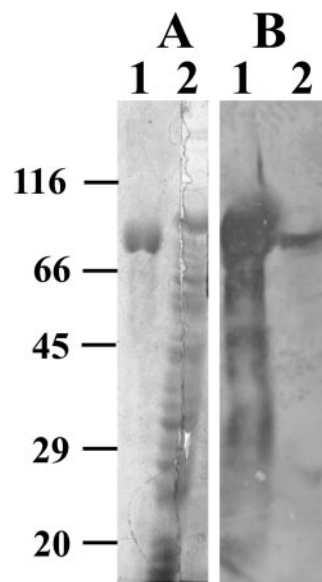
FIG. 4. SDS-PAGE and Western blot identification of purified histidine-tagged recombinant YaeT. (A) Coomassie blue-stained SDS-PAGE gel. (B) Western blot analysis using rabbit anti-H-YaeT (1:50,000). Lane 1, nickel affinity-purified H-YaeT; lane 2, whole-cell lysates of E. coli strain MC1061.
