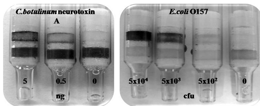
FIG. 3. AICC columns used for sensitive detection of botulinum neurotoxin complex A and E. coli O157. The limit of detection for the botulinum type A neurotoxin complex AIC assay was 0.5 ng. The limit of detection for the E. coli AICC assay was 500 CFU. Each column contained a negative-control frit toward the top of the column, a specific measurement filter in the middle, and a positive-control frit toward the bottom of the column. Measurement frits were separated with a spacer frit absorbed with 1% (wt/vol) BSA.
